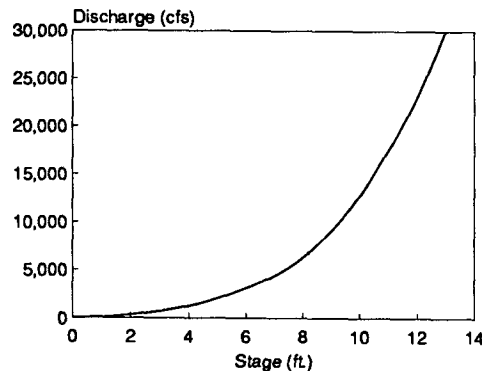
Figure 12. Example of a rating curve from the San Pedro River, Arizona. The table allows researchers to use stage information (vertical height of water) to determine flow at a transect site.
