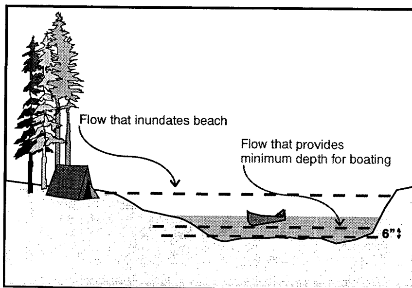
Figure 14. Simplified case where hydraulic geometry modeling can be used to identify flows that provide minimum depths for boating or that would inundate camping beaches.
