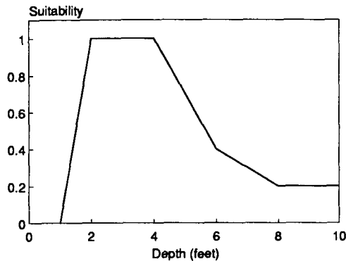
Figure 36. Depth suitability criteria for boating. Minimum depth is 1 foot and optimum is 2-4 feet, although depths from 6-10 feet are acceptable.
