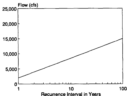
Figure 9. A peak flow analysis (also known as a flood frequency analysis) shows how often floods of a certain size are likely to occur. Data come from the Dolores River prior to construction of McPhee Dam.
